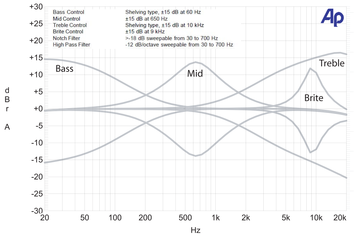
Tone Control Response for Series II Amps
